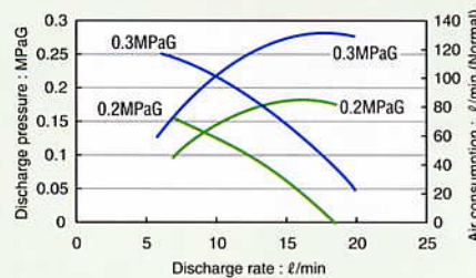
Performance Curves for PS-E 20MA (at 50°C)
