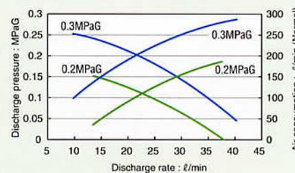
Performance Curves for PS-E 40MA (at 50°C)
