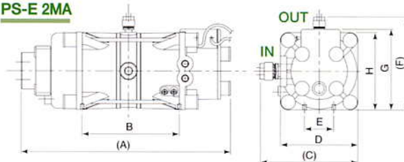
DIMENSIONS (mm)
