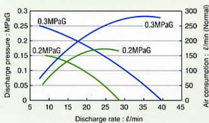
Performance Curves for PS-E 40MA (at 20°C)
