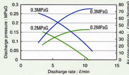
Performance Curves for PS-E 10MA (at 50°C)
