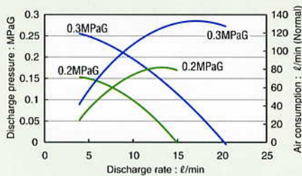
Performance Curves for PS-E 20MA (at 20°C)
